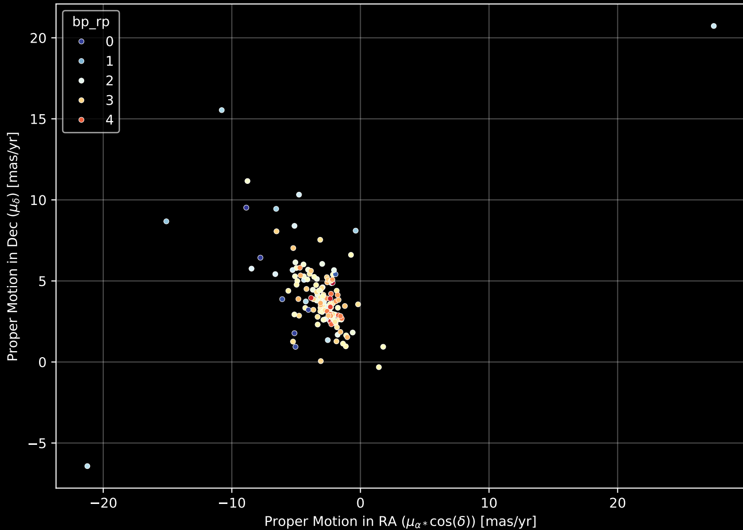
APOGEE DR17 Field: [263-03] Proper Motion Diagram (n= 139)
