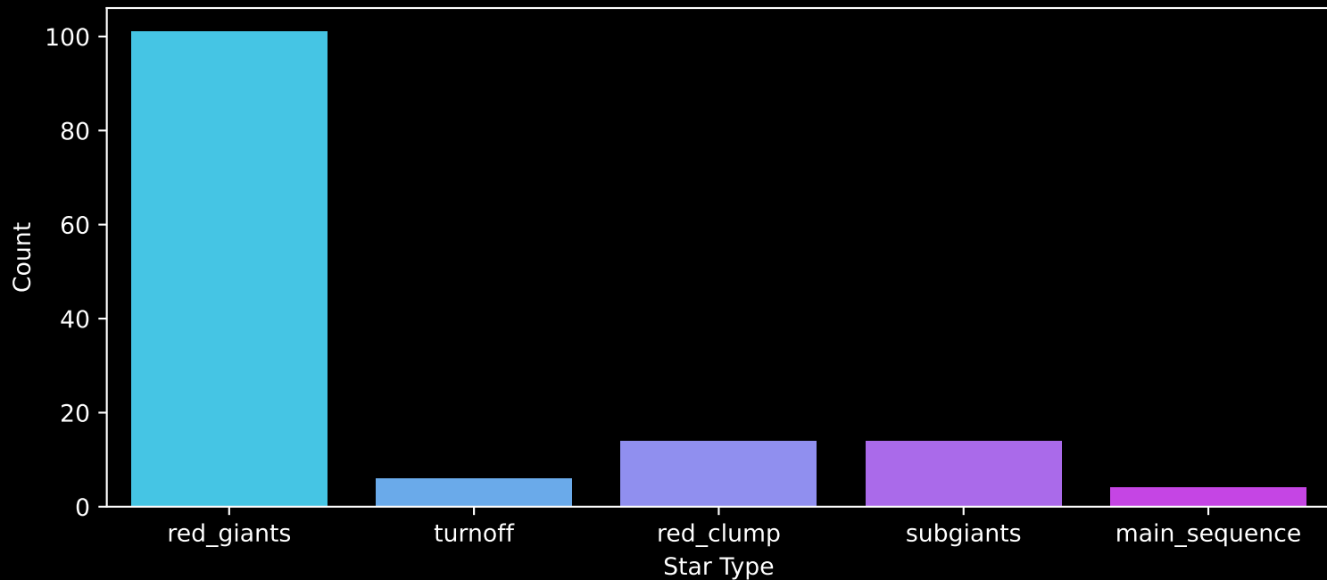
APOGEE DR17 Field: [263-03] Count plot of Star Type
