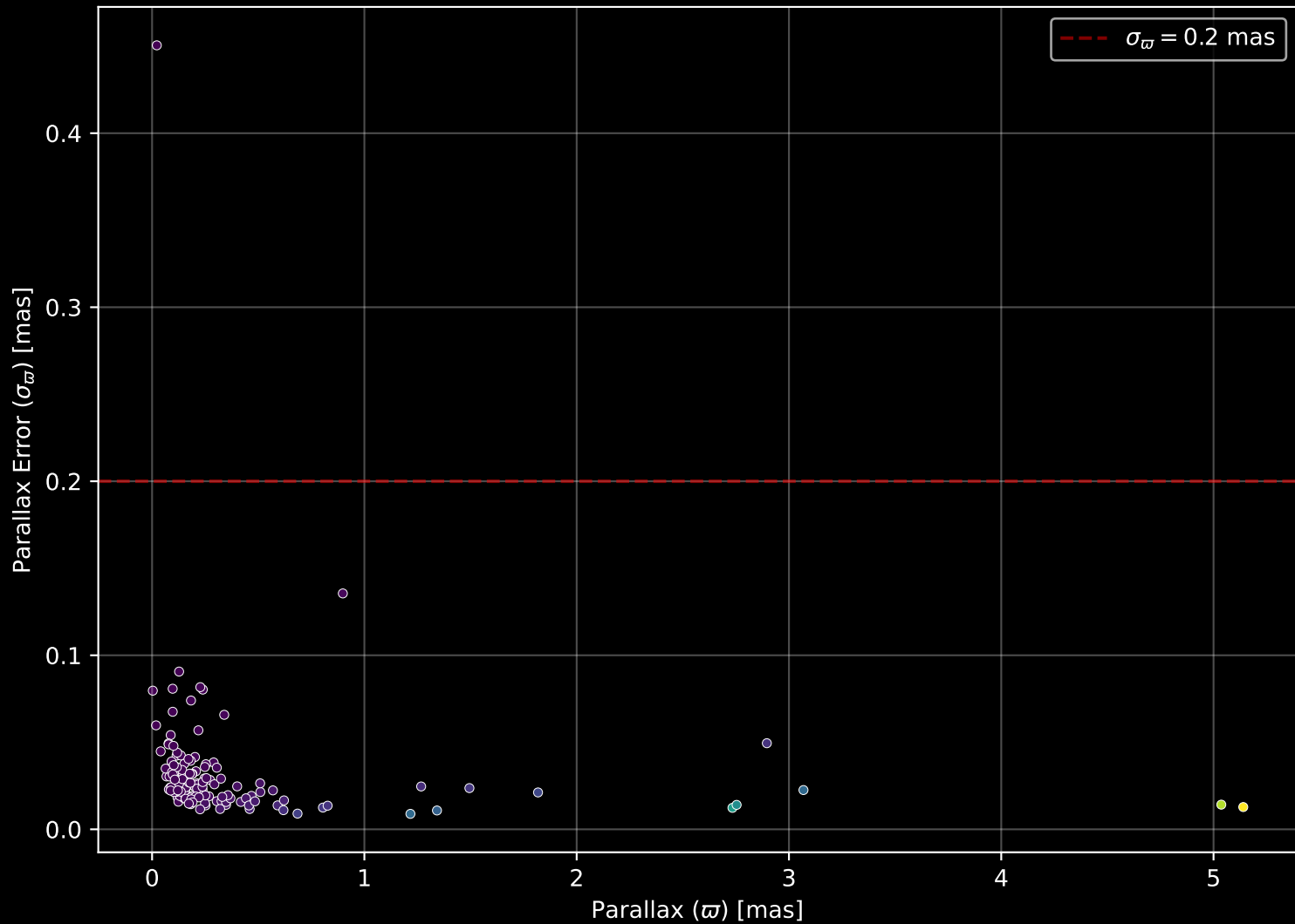
APOGEE DR17 Field: [263-03] Parallax Quality (n= 139)
