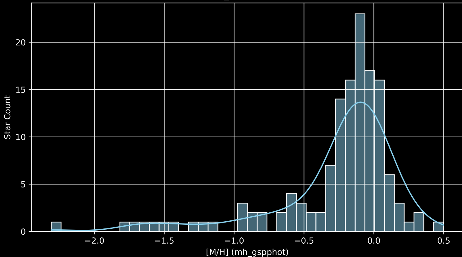
APOGEE DR17 Field: [263-03 [M/H] (mh_gspphot) (n= 136)
