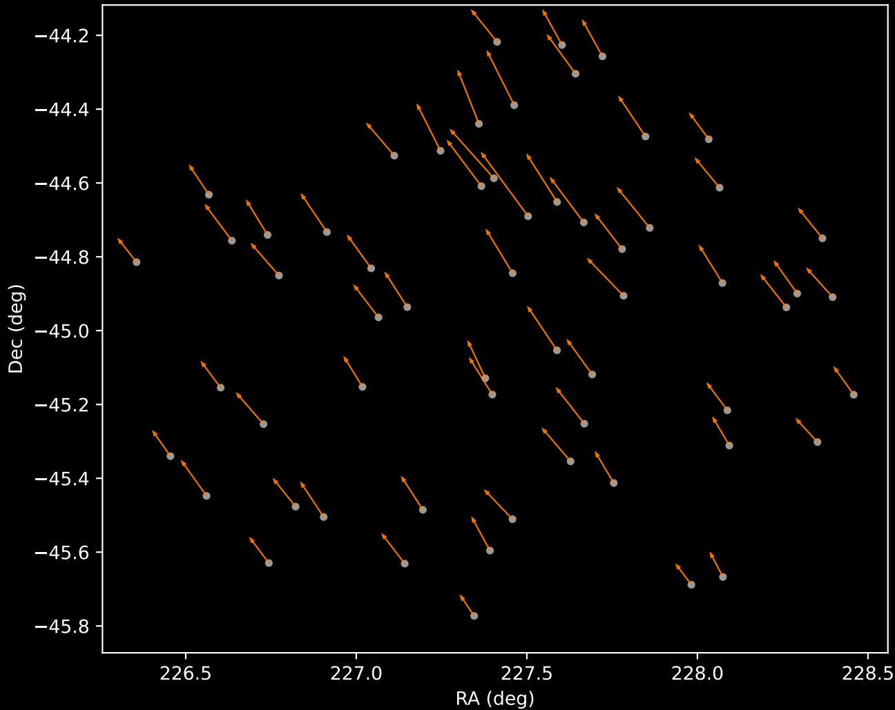
APOGEE DR17 Cluster 2 Proper Motion Vectors (n=60)
