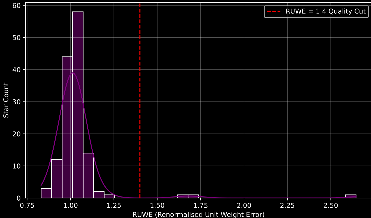
GAPOGEE DR17 Field [263-03] RUWE Distribution (n= 137)
